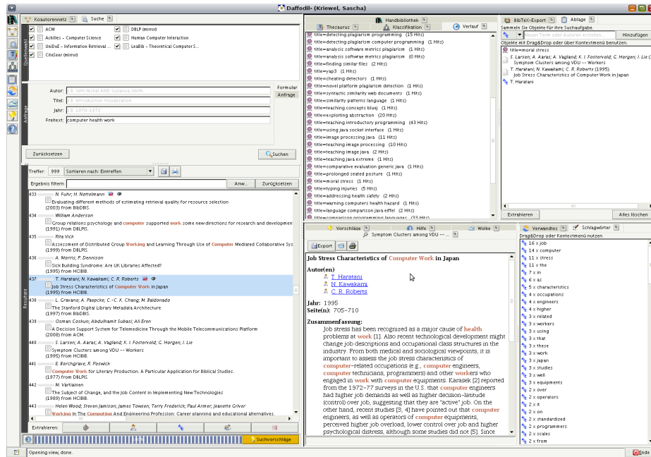
Fig. 1. The DAFFODIL desktop: search tool (left), search history (top center), clipboard (top right), detail view (bottom center), and Related Terms (bottom right)
